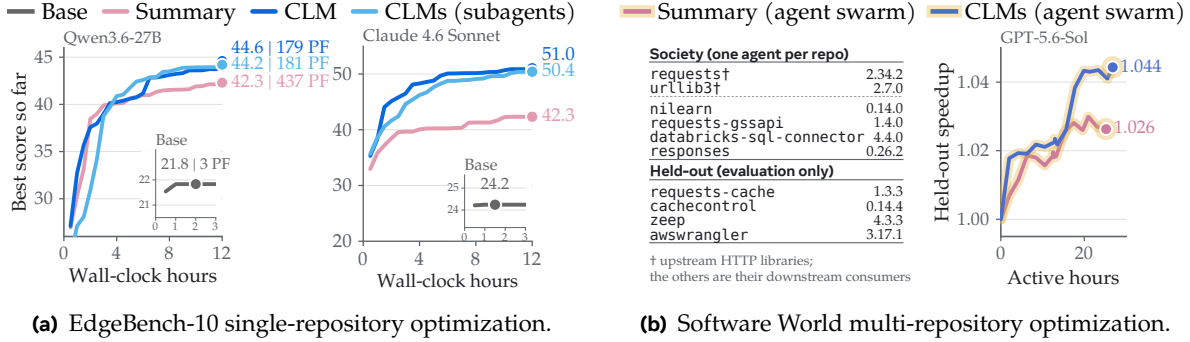
Figure 6 CLMs outperform Codex-style summary harness on long-horizon repository optimization. (a) EdgeBench-10 with a 32K context budget. Curves show best-of-three scores over 12 hours for Qwen3.6-27B and Claude 4.6 Sonnet; end labels show final scores and, for Qwen3.6-27B, mean compute per trial (PF = prefix-reuse PFLOPs). (b) Software World with GPT-5.6-Sol and a 272K context budget. Six agents jointly optimize interdependent repositories and are evaluated on four unseen downstream packages; the right panel shows geometric-mean speedup over 17 evaluation tasks.
