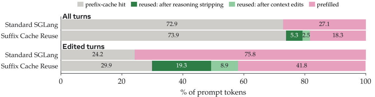
Figure 12 Suffix Cache Reuse also benefits standard chat serving. On BrowseComp-Plus, SCR reuses cached states not only after model-driven context edits but also after reasoning tokens are stripped from prior turns in standard chat endpoints. Results use Qwen3.6-27B on 830 questions with K = 6 .
