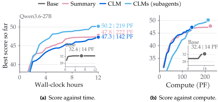
Figure 19 EdgeBench-10 single-repository optimization with a 128K context budget. Qwen3.6-27B, ten tasks, three seeds. End labels give final scores and mean compute per trial (PF = prefix-reuse PFLOPs); insets show the base harness.
