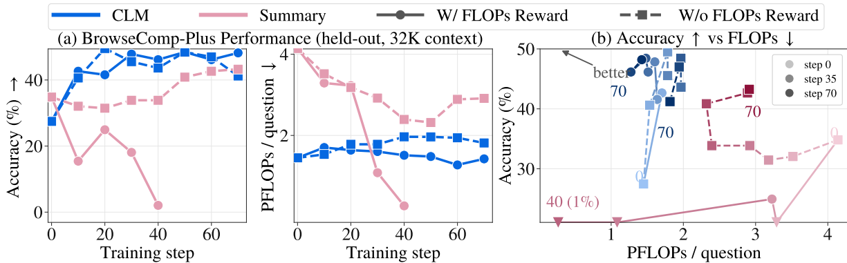
Figure 21 RL training curves. Qwen3.5-9B trained on OpenResearcher and evaluated on BrowseComp-Plus with a 32K context limit, through training step 70. (a) Accuracy and prefix-reuse PFLOPs per question against training step. (b) Accuracy against compute, shaded from light to dark by training step.
