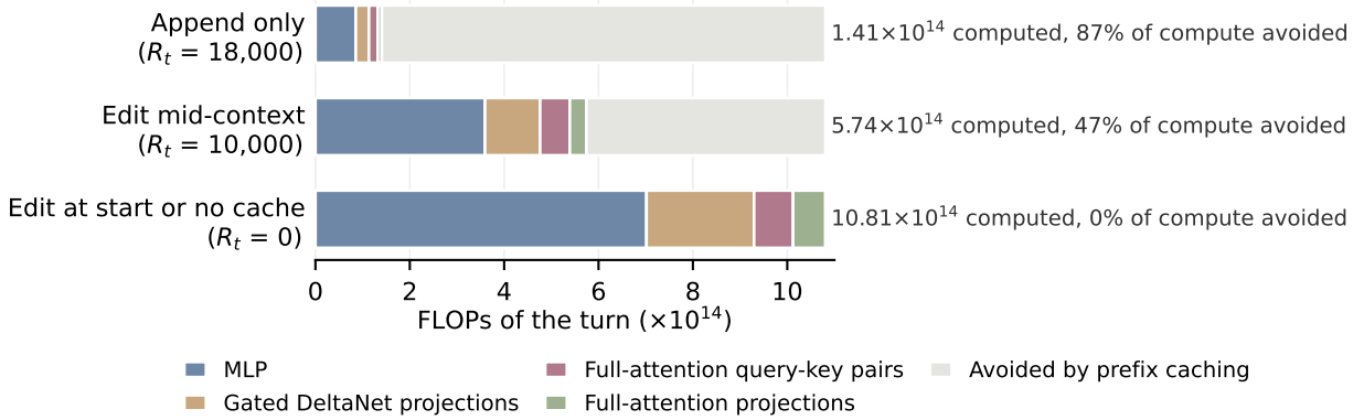
Figure 14 FLOPs of one Qwen3.6-27B turn for illustrative lengths ( P_t = 20,000 , G_t = 500 ) and three reusable-prefix lengths R_t . Colors split the FLOPs actually computed by operation; gray shows the additional computation that would be required without prefix caching.
