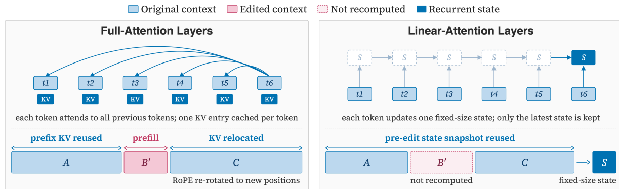
Figure 10 Suffix Cache Reuse for full attention layers and linear attention layers.
