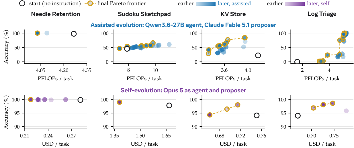
Figure 20 Evolving context-management skills on ContextBench (32K budget), all four tasks. Assisted evolution (top): Qwen3.6-27B serves as the agent, while Claude Fable 5.1 proposes the skills; the x-axis shows prefix-reuse PFLOPs per task over solved runs. Self-evolution (bottom): Opus 5 serves as both the agent and the skill proposer; the x-axis shows gateway cost per task in USD. Skills are proposed based on training-split rollouts and never use the held-out evaluation set.
