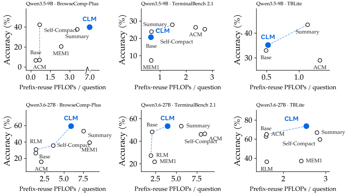
Figure 17 Qwen3.5-9B and Qwen3.6-27B. Accuracy against compute for Qwen3.5-9B (top) and Qwen3.6-27B (bottom) on BrowseComp-Plus, TerminalBench 2.1 and TBLite with a 32K context limit. Cost is prefix-reuse PFLOPs per question; dashed lines indicate the Pareto frontier.
