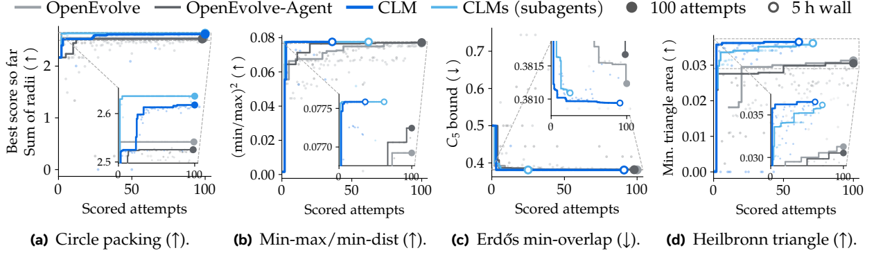
Figure 18 Best-so-far score versus evaluator-scored attempts on four open optimization problems. All runs use Claude 4.6 Sonnet with a 32K context limit and stop after 100 attempts or five hours. Lines show the best score so far, dots individual scored candidates, and insets the final-score range.
