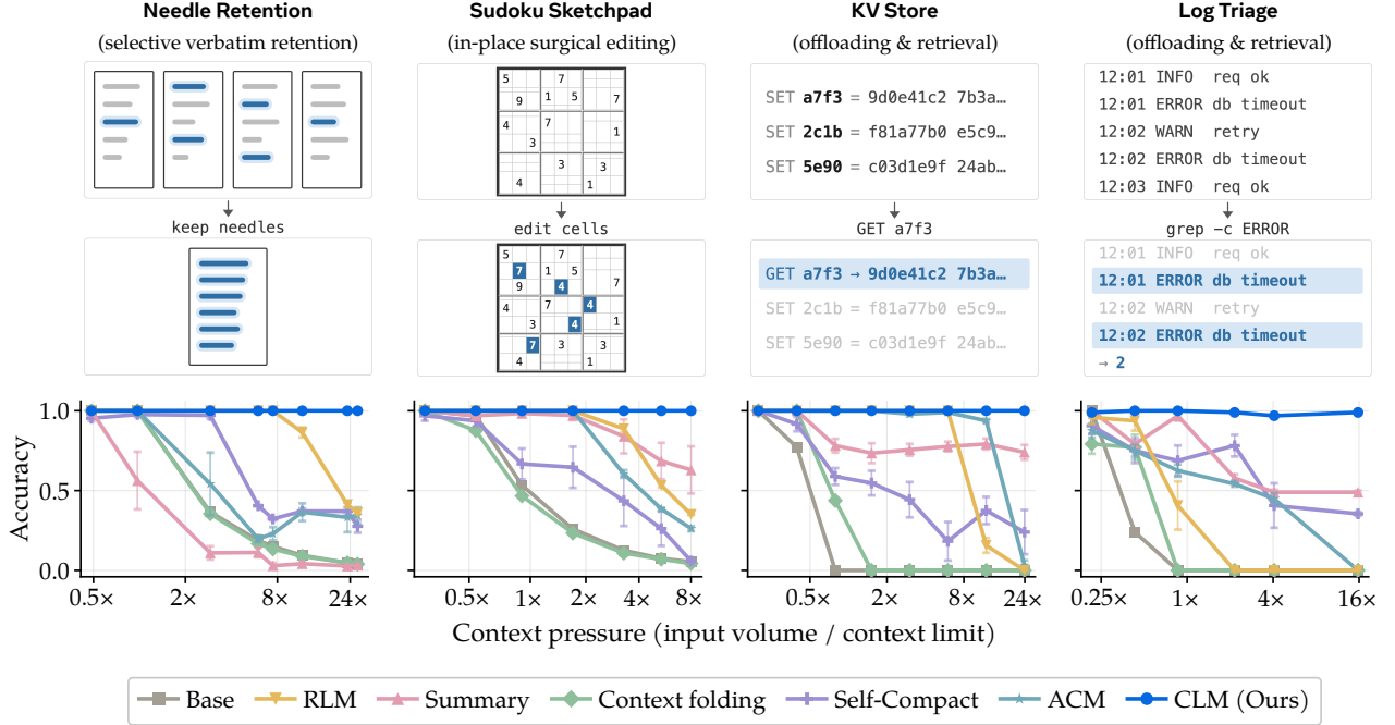
Figure 2 Illustration of the four tasks in ContextBench and a performance comparison of CLM against baselines using GPT-5.4 with a 32K context limit.
