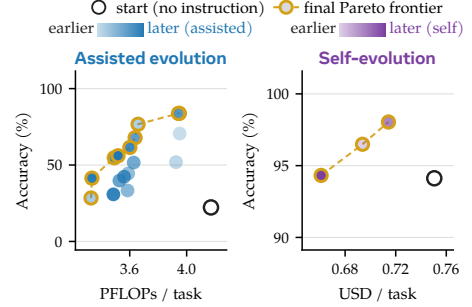
Figure 8 Textual evolution for CLMs on KV Store (32K budget). Assisted evolution uses Qwen3.6-27B with Claude Table 5.1 as proposer; self-evolution uses Opus 5 for both roles.
