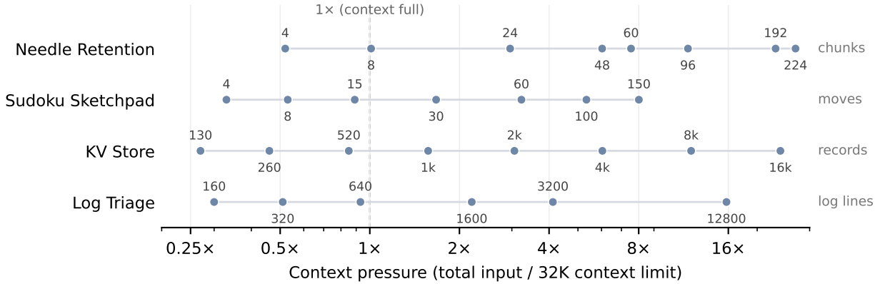
Figure 15 Context pressure of every ContextBench level. Each row varies one generator setting (unit at right); the label on each point is its value. Total input is every message the environment pushes over the episode, including the task instruction and, for Sudoku, the board once per move, counted in o200k tokens; pressure is total input divided by 32,768.
