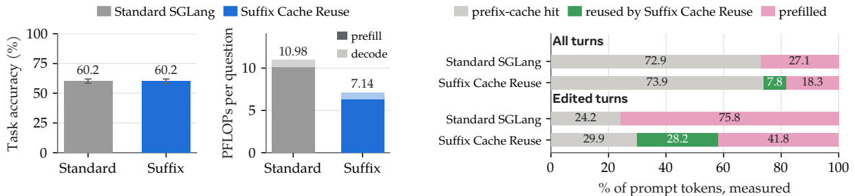
Figure 9 Comparison of Suffix Cache Reuse and standard SGLang serving on BCP with Qwen3.6-27B. Left: Task accuracy and prefix-reuse FLOPs per question. Right: Server-side compute decomposition, showing the fraction of prompt tokens by compute type across all turns and turns following context edits.
