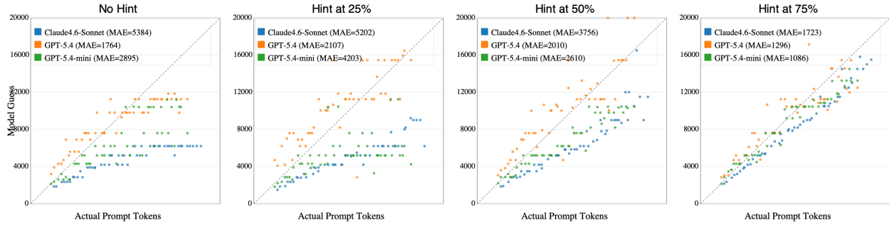
Figure 22 Context length awareness. Each point compares a model’s estimated context length with the provider-reported prompt length for the same 50 inputs. Panels vary the available hint: none or a token-count anchor at 25%, 50%, or 75% of the input. The dashed line indicates perfect calibration; legend values report mean absolute error (MAE) in tokens.
