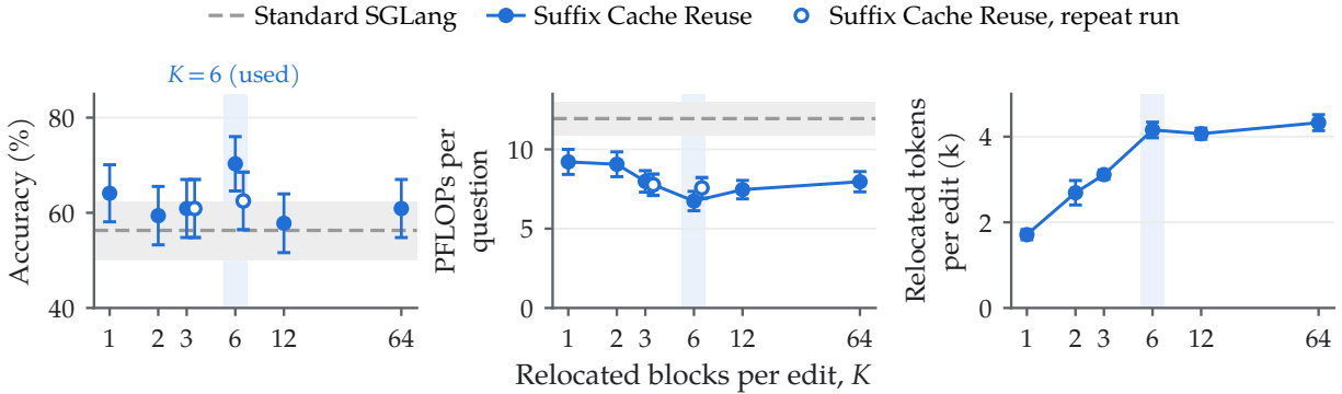
Figure 11 Small-scale sensitivity study of relocated spans per edit, K . Results on 64 BrowseComp-Plus questions with Qwen3.6-27B. Left: task accuracy. Middle: prefix-reuse PFLOPs per question. Right: relocated tokens per edited request. Dashed lines show standard SGLang; hollow markers show a repeat run; the shaded column marks K=6 , used elsewhere. Error bars show \pm 1 standard error across questions; the gray band shows \pm 1 standard error for standard SGLang.
