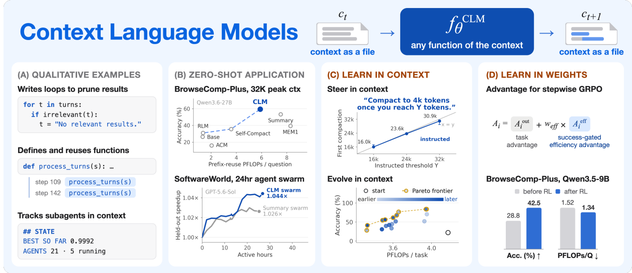
Figure 1 Context Language Models (CLMs) natively manage their own context by treating context as a file. CLMs work out of the box and can be further improved through in-context learning and reinforcement learning. (a) Qualitative examples of creative context-management behaviors introduced by CLM. (b) Out of the box, CLMs improve performance at lower cost on BrowseComp-Plus, a deep-research benchmark, and Software World, where an agent swarm jointly optimizes six interdependent repositories. (c) CLMs can follow textual instructions to adopt corresponding context-management strategies (top) or evolve better strategies through a skill-evolution loop on ContextBench (bottom). (d) CLMs can explore and internalize context-management strategies through online reinforcement learning. By using a success-gated efficiency advantage for stepwise GRPO, we improve both accuracy and efficiency for CLMs simultaneously.
