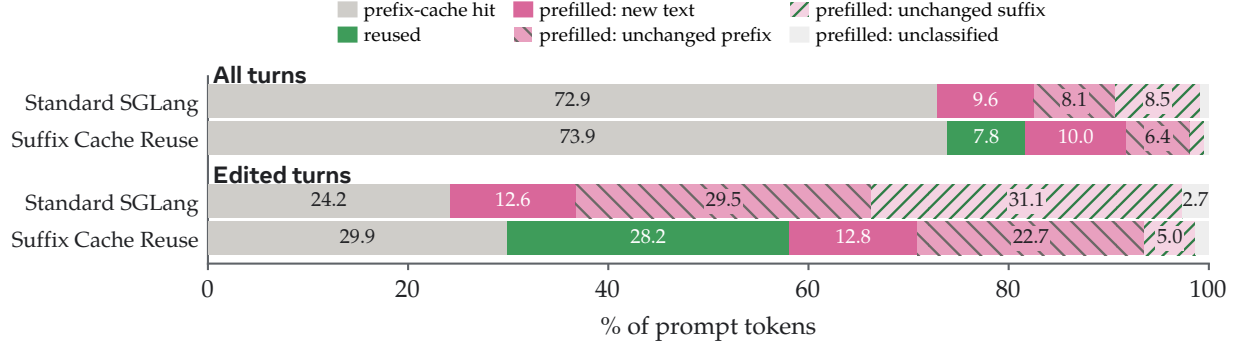
Figure 13 Remaining re-prefill under Suffix Cache Reuse on BrowseComp-Plus. SCR removes most re-prefilling of unchanged suffix tokens, while substantial unchanged-prefix prefill remains due to the current hybrid-model caching behavior in SGLang. Same runs as Figure 12.
