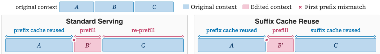
Figure 4 Comparison of standard serving and Suffix Cache Reuse (SCR). Standard serving reuses only prefix-matched cache, while SCR reuses cached states for all surviving tokens, reducing re-prefilling.
