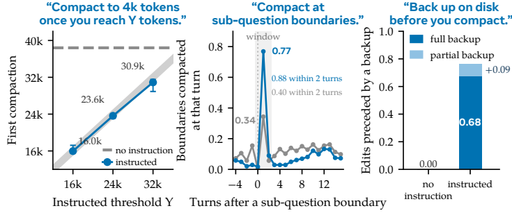
Figure 7 One sentence in the prompt changes the context-management policy. Natural-language instructions steer compaction timing, semantic boundaries, and backup behavior. Gray denotes no instruction and blue the instructed setting; exact prompts are in Appendix E.
